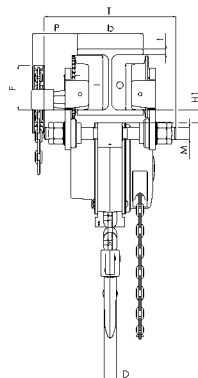
Model Yalelift ITG, 500 - 3000 kg, single fall
