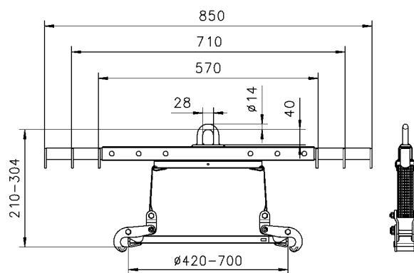
Model TFA-TR
