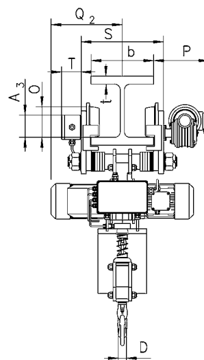
Model CPE/CPEF with integrated electric trolley, 10000 kg
