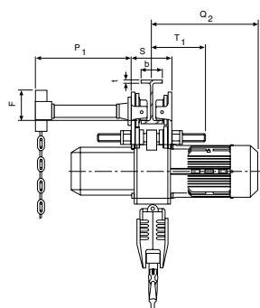
Model CPE/CPEF with integrated manual push or geared trolley
